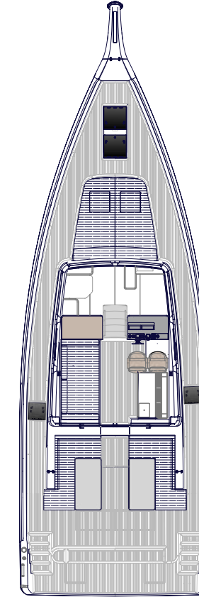
Main Deck
